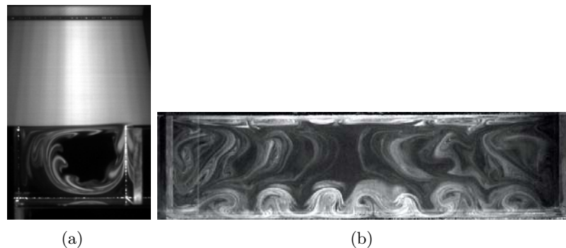
Figure 2. Smoke visualization for a cavity geometry L/H = 1.5 , S/H = 6 and for a typical Reynolds number \mathcal{R}_H \approx 3000 . (a) Front view of the longitudinal plane (x, y) , (b) top view of the spanwise plane (x, z) located at y/H = -0.3 inside the cavity.
